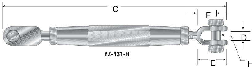
Antenna Fitting - US Navy Ship Communications Tower
