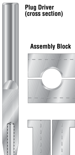
ASSEMBLY KITS FOR INDIVIDUAL WIRE ROPE
