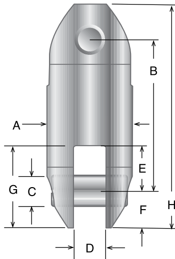
7200 SERIES 90-DEGREE CONNECTORS - CLEVIS/CLEVIS
